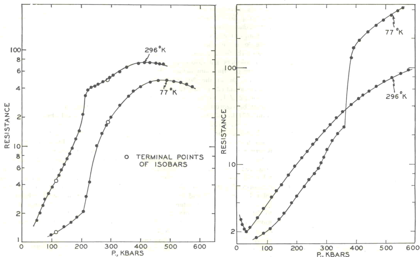
Fig. 9 (left). Resistance plotted against pressure for rubidium. Fig. 10 (right). Resistance plotted against pressure for potassium.
